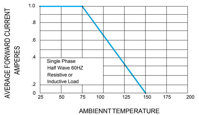
FIG.4 -- FORWARD DERATING CURVE
